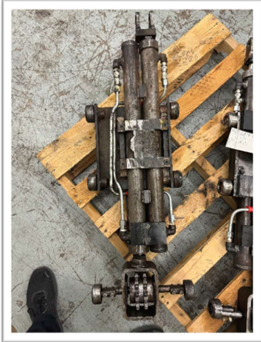
Figure 4 (Top) Cart Flipper Assembly
