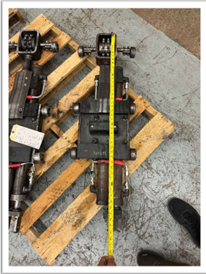
Figure 2 (Bottom) Cart flipper assembly with vertical measurement (Roughly 44 in long )
