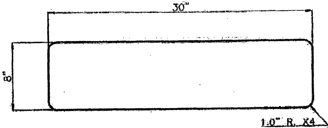
Cutting Diagram – Sign Blank
